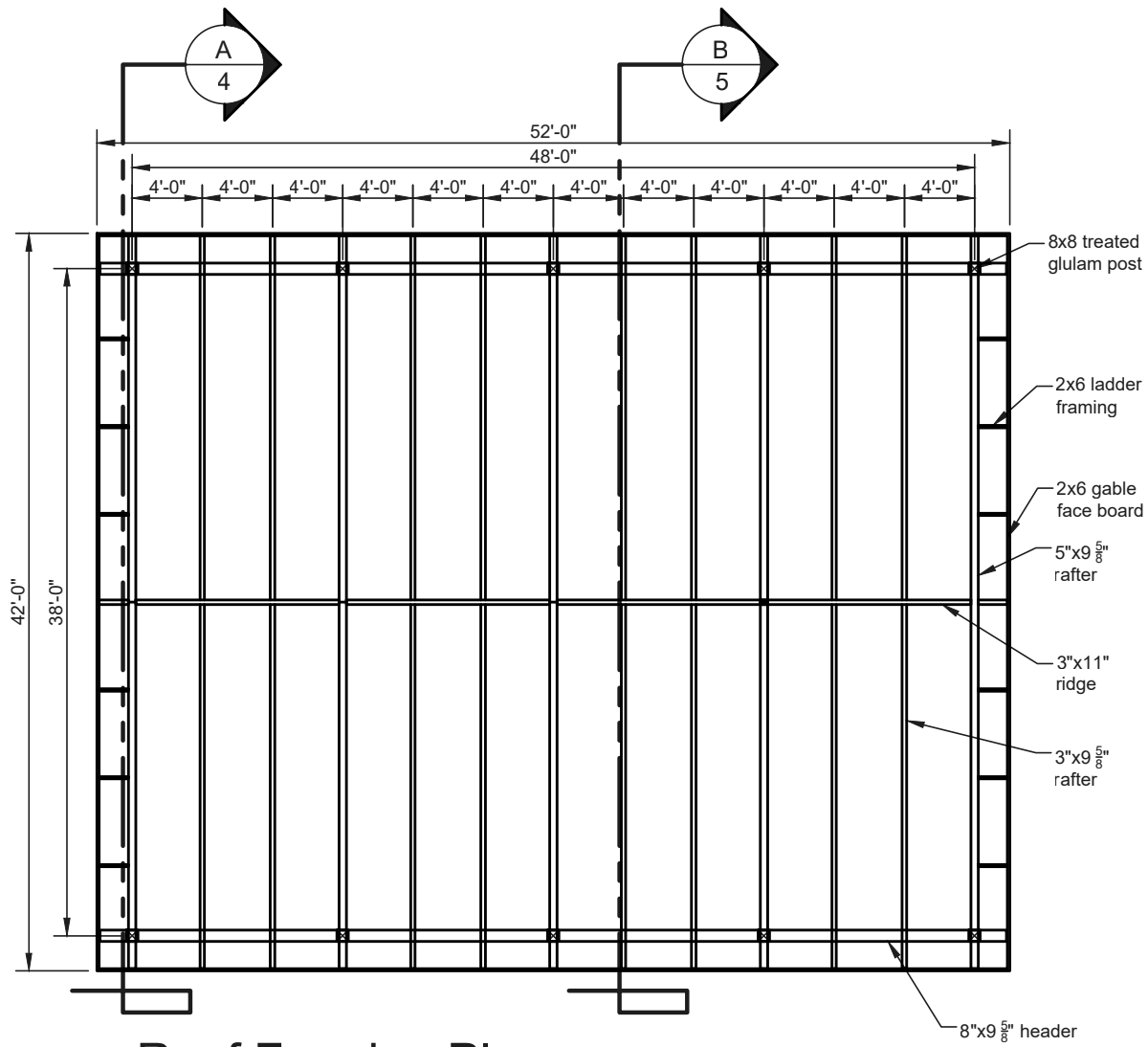
Roof Framing Plan NTS
