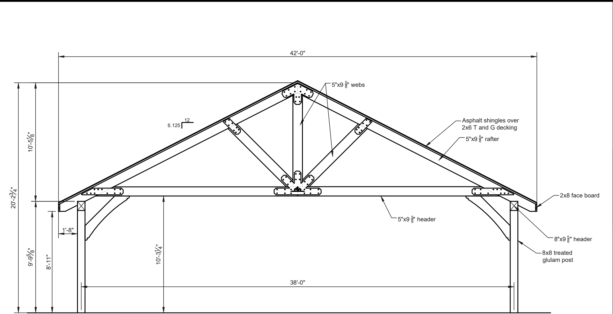
Cross Section A/4 NTS
