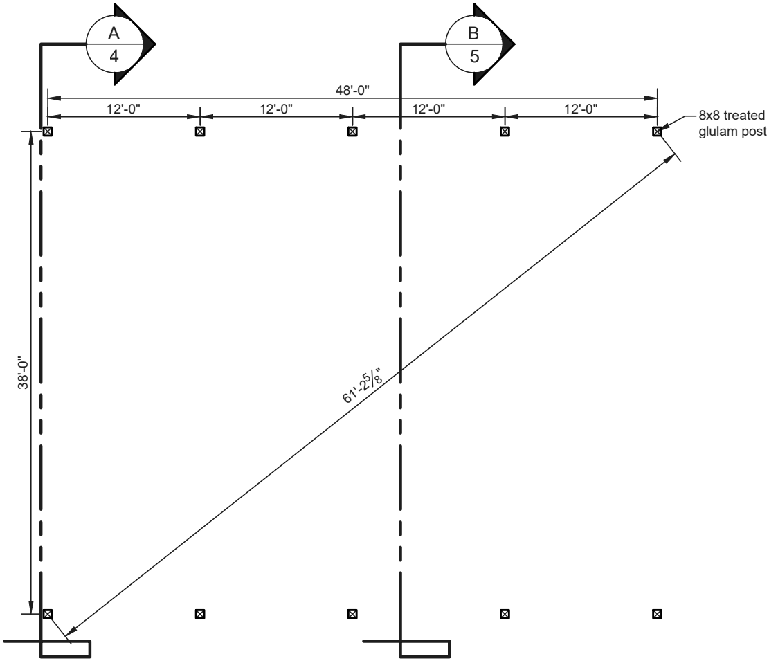
Post Layout Plan NTS
